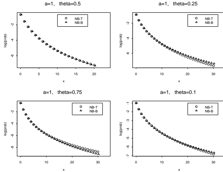
Figure 1.3: Plots of the probability function in log scale of the NB-T distribution for \alpha = 1 and \theta = 0.5, 0.25, 0.75, 0.1 superimposed by plots of the Generalized Waring (NB-B) distribution with the same mean.
