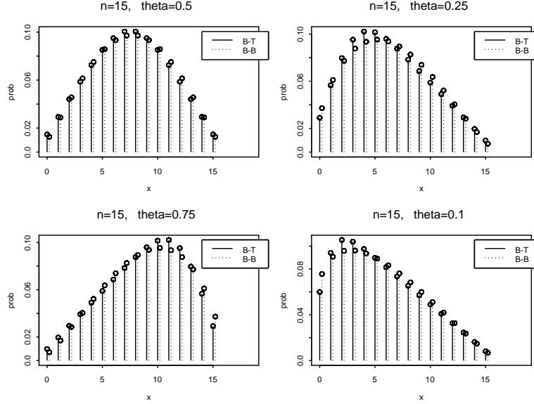
Figure 1.2: Plots of the probability function of the B-T distribution for n = 15 and \theta = 0.5, 0.25, 0.75, 0.1 superimposed by plots of the B-B with the same mean and variance.
