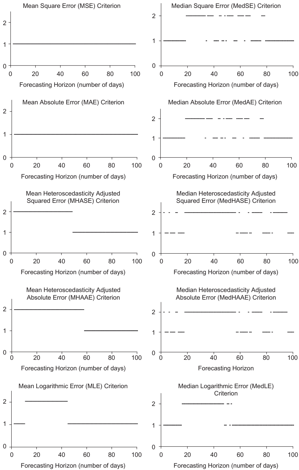
Fig. 2(a). The plots indicate whether the ARCH models selected by the SPEC algorithm achieve the lowest value of the evaluation criterion, for a forecasting horizon ranging from one day to 100 days ahead. The value 2 indicates that the ARCH model selected by the SPEC algorithm achieves the lowest value for the corresponding criterion and the specific forecasting horizon. The value 1 indicates the opposite. The realized volatility measure is expressed as in Equation 12. The evaluation criteria are the mean and the median values of the functions defined by Equations 14–18
