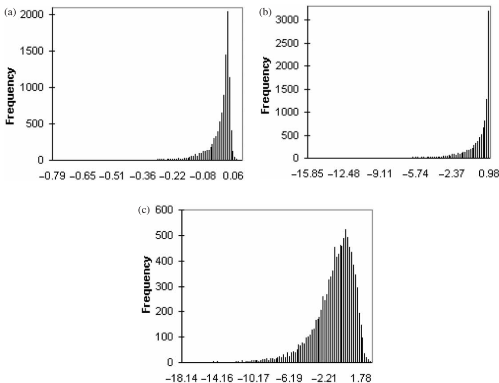
Fig. 1(a). Histogram of \hat{\sigma}_{t+1|t}^2 - y_{t+1}^2 from an AR(1)GARCH(1,1) simulated process, (b) Histogram of 1 - y_{t+1}^2 / \hat{\sigma}_{t+1|t}^2 from an AR(1)GARCH(1,1) simulated process, (c) Histogram of \ln(y_{t+1}^2 / \hat{\sigma}_{t+1|t}^2) from an AR(1)GARCH(1,1) simulated process
