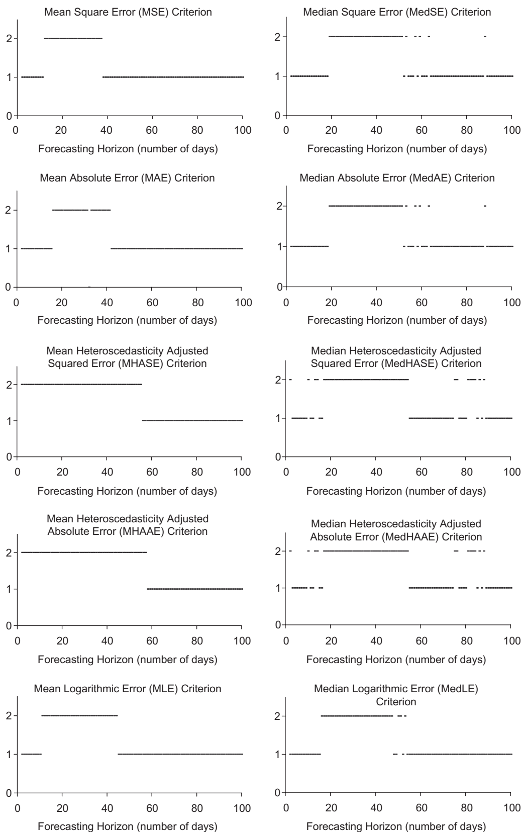
Fig. 2(b). The plots indicate whether the ARCH models selected by the SPEC algorithm achieve the lowest value of the evaluation criterion, for a forecasting horizon ranging from one day to 100 days ahead. The value 2 indicates that the ARCH model selected by the SPEC algorithm achieves the lowest value for the corresponding criterion and the specific forecasting horizon. The value 1 indicates the opposite. The realized volatility measure is expressed as the square root of Equation 12. The evaluation criteria are the mean and the median values of the functions defined by Equations 14–18
