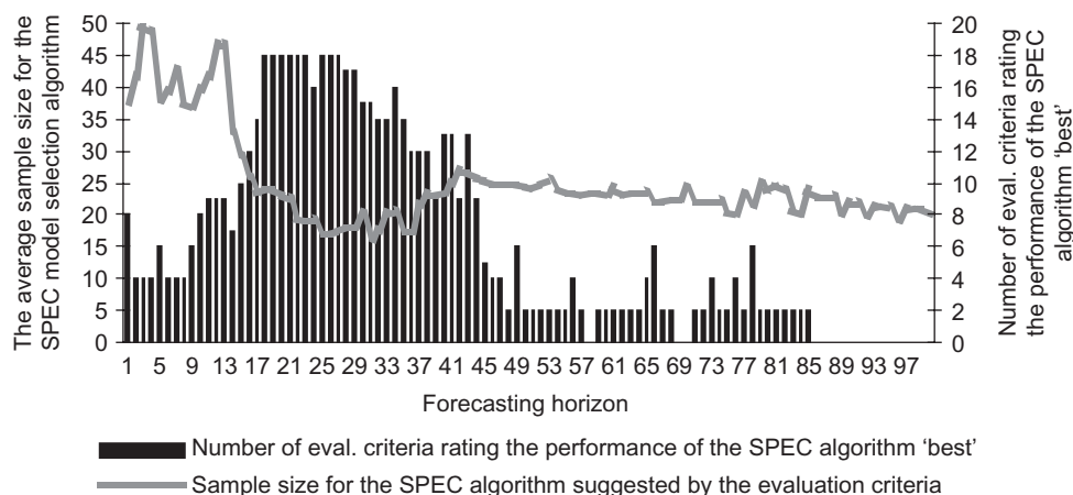
Fig. 3. Sample size of the SPEC model selection algorithm, suggested by the evaluation criteria
